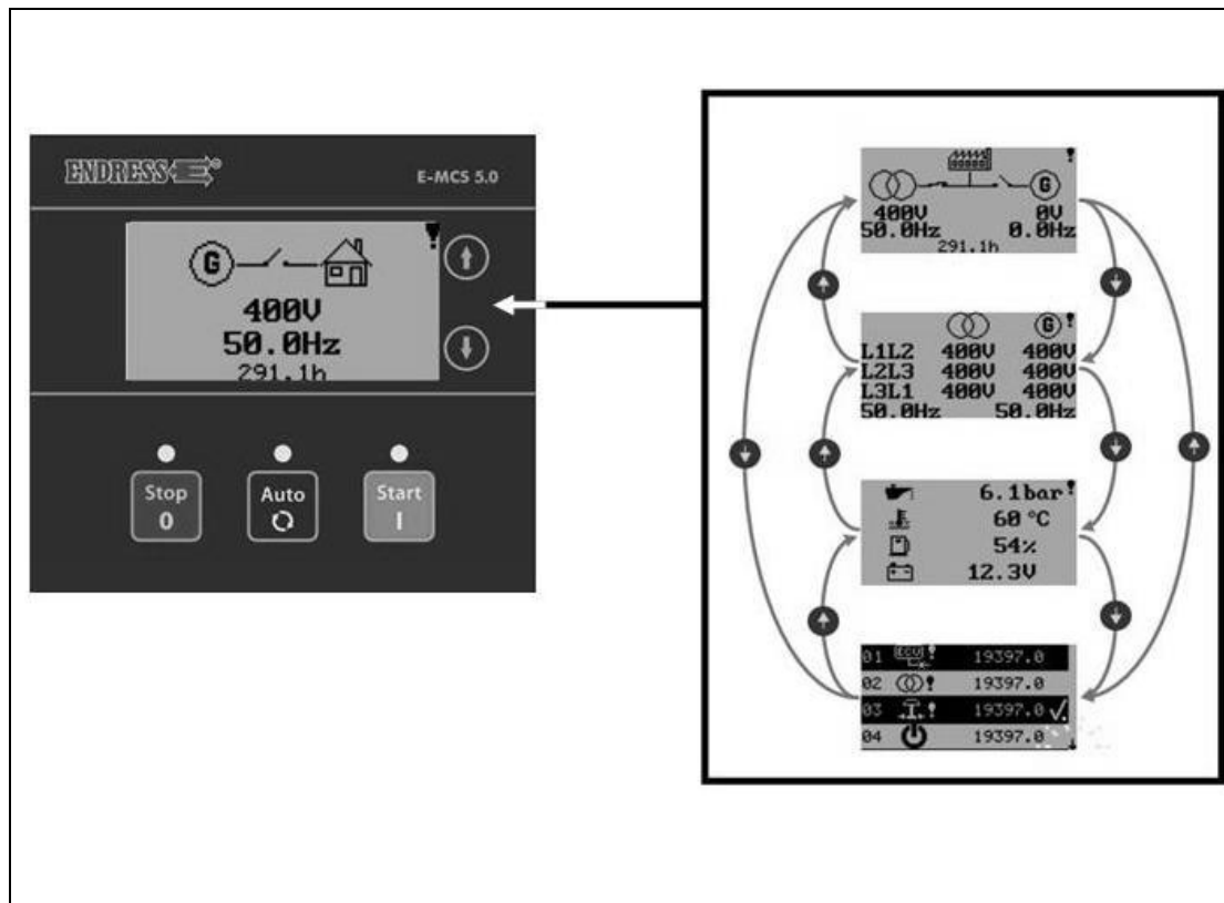
Abb. 6-1: Statusabfragen E-MCS 5.0
